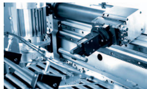
Timed conveyor system with V-supports for preformed shaft parts of various shapes.
