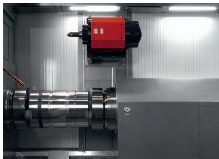
Powerful counter-spindle. The counter-spindle and main spindle are identical when it comes to their specifications and construction. Thus, it is possible to machine even more complex parts in one setting. This results in more flexibility, increased productivity and lower storage costs for the customer.
