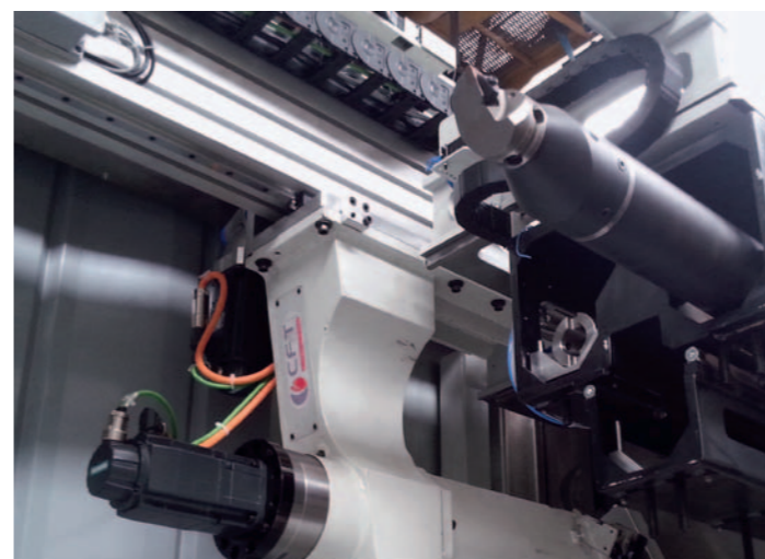
XL magazine. Equipped with a 3-positions pick-up magazine, it includes tools up to a length of 1000 mm
