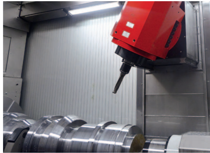
Milling spindle. For stable, precise and flexible drilling and milling operations. Up to 80 kW and 630 Nm of torque and 10000 rpm. Sealing air, internal HP coolant with 40 bar and externally with 14 bar and a 1400 liter paper band filter system as standard (80 bar option). The B-axis can be used at any angle or with an indexed B-axis in 2.5° steps.
