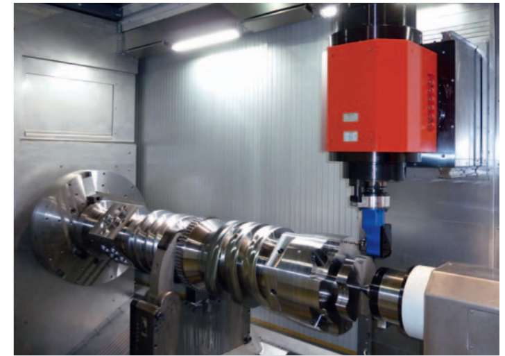
Machining options. From an angular tool holder to an additional U-axis – all machining processes are possible and feasible in a customised way.
