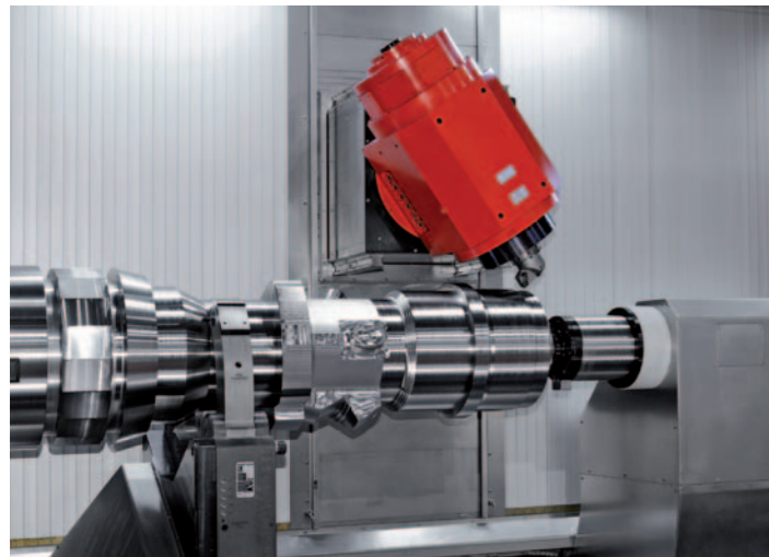
Tailstock. The tailstock is 100% programmable using the control. With the high-quality and precisely-dimensioned MK6 quill, all operations can be supported or extended with the counter spindle thanks to the machine modular construction.
