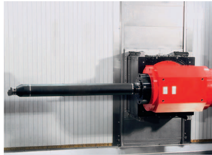
Turning operations. External or internal turning operations are possible with the stable spindle in 3° step. Optionally, the vibration-damped boring bar can be equipped up to a length of 1000 mm and with a 3-positions (stations) pick-up magazine.
