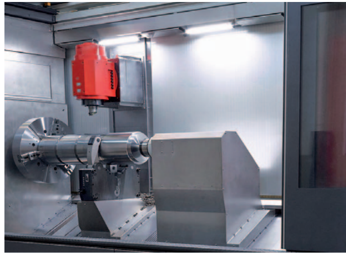
Main spindle. For turning and milling operations, equipped with 84 kW and 6400 Nm torque. Sealing air, working area coolant and programmable clamping pressure are standard features on the Hyperturn 200. One or more programmable NC steady rest can assist the processing.
