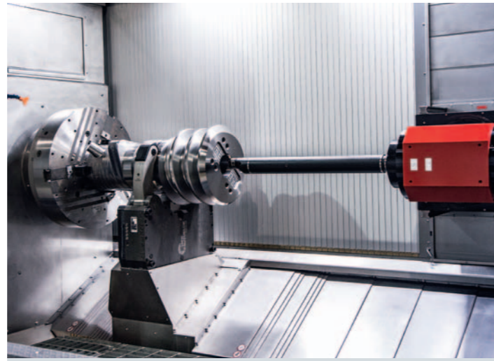
Boring bar: Boring bar with vibration absorption featuring a diameter of 100 x 100 mm for internal turning operations. There are three specifically dimensioned tools available.
